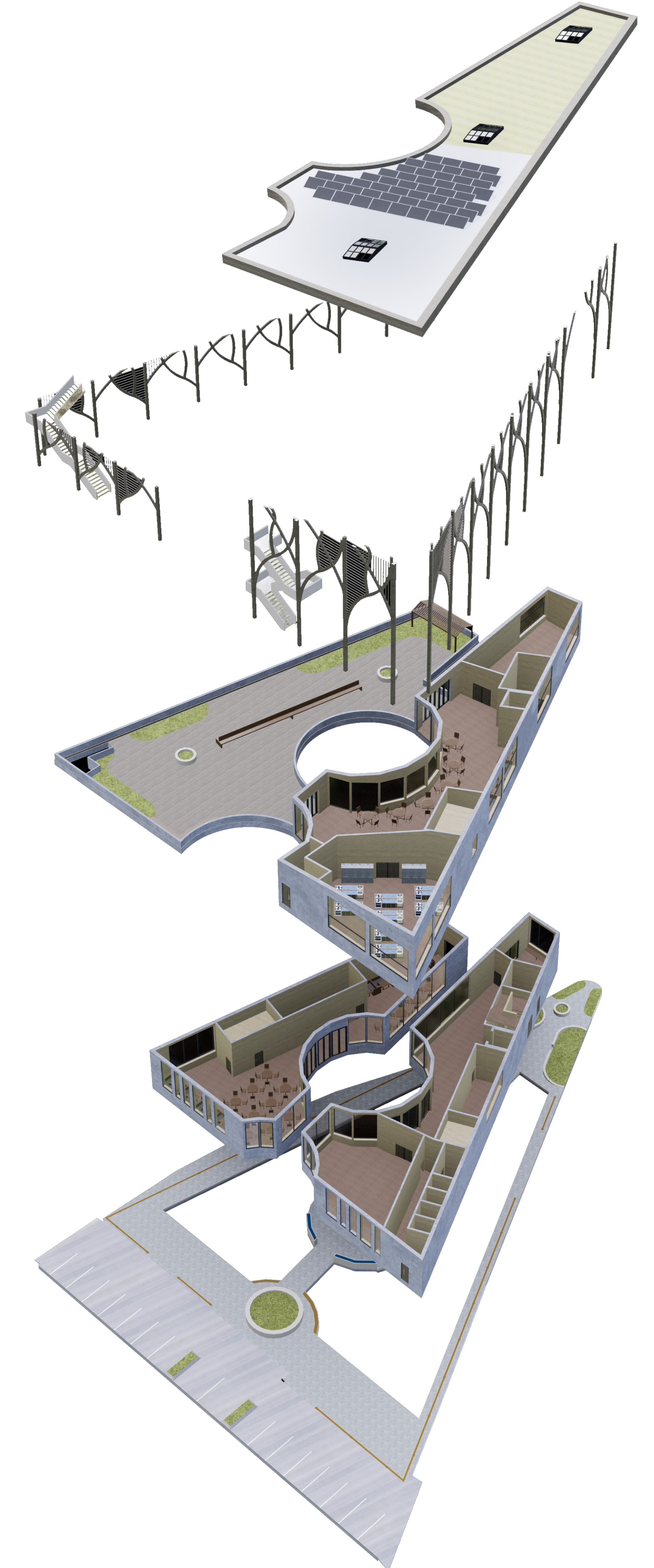
Exoskeleton 3D Fitting
