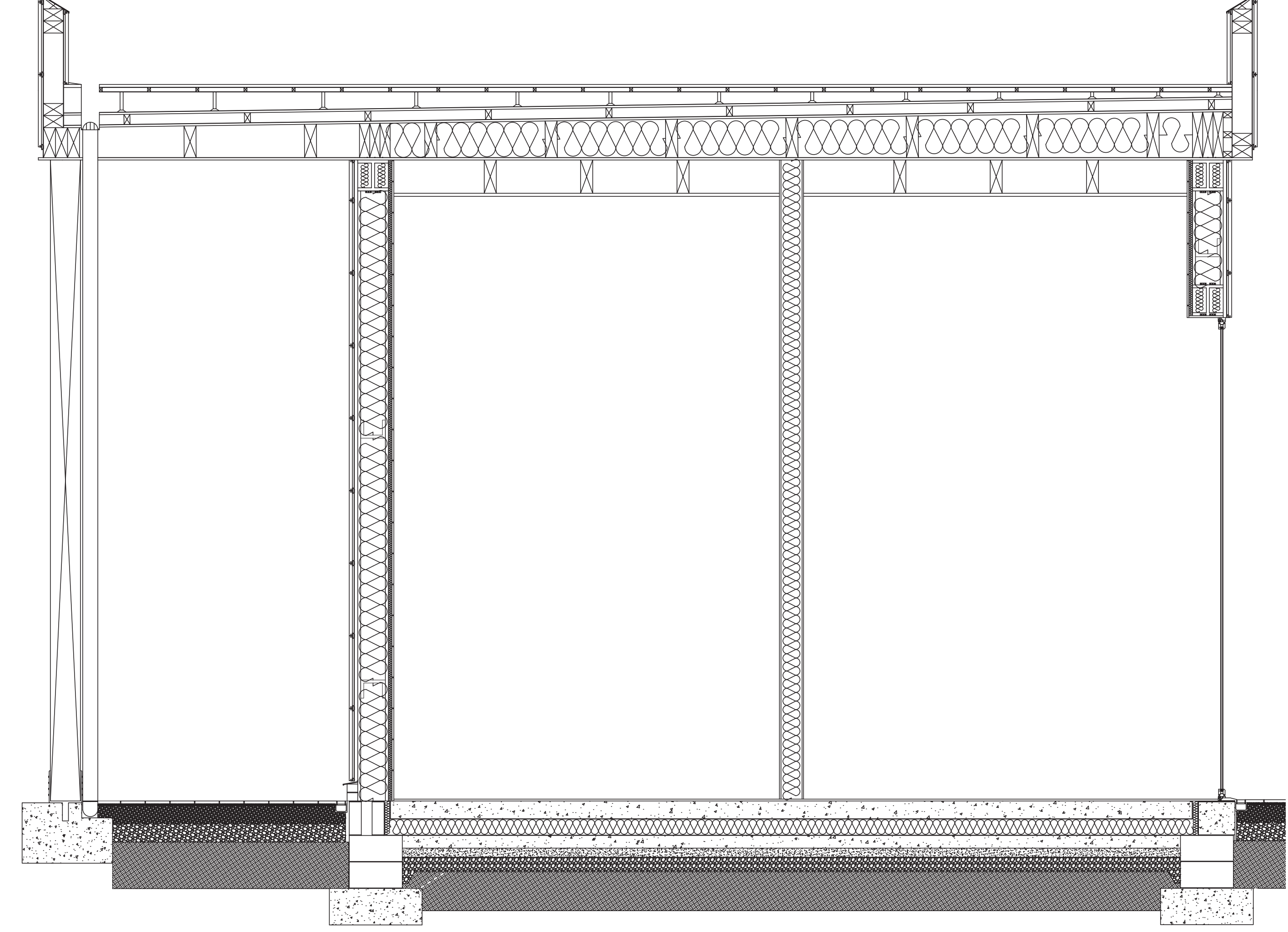
Cafe Building Detail 1:20 @ A2
