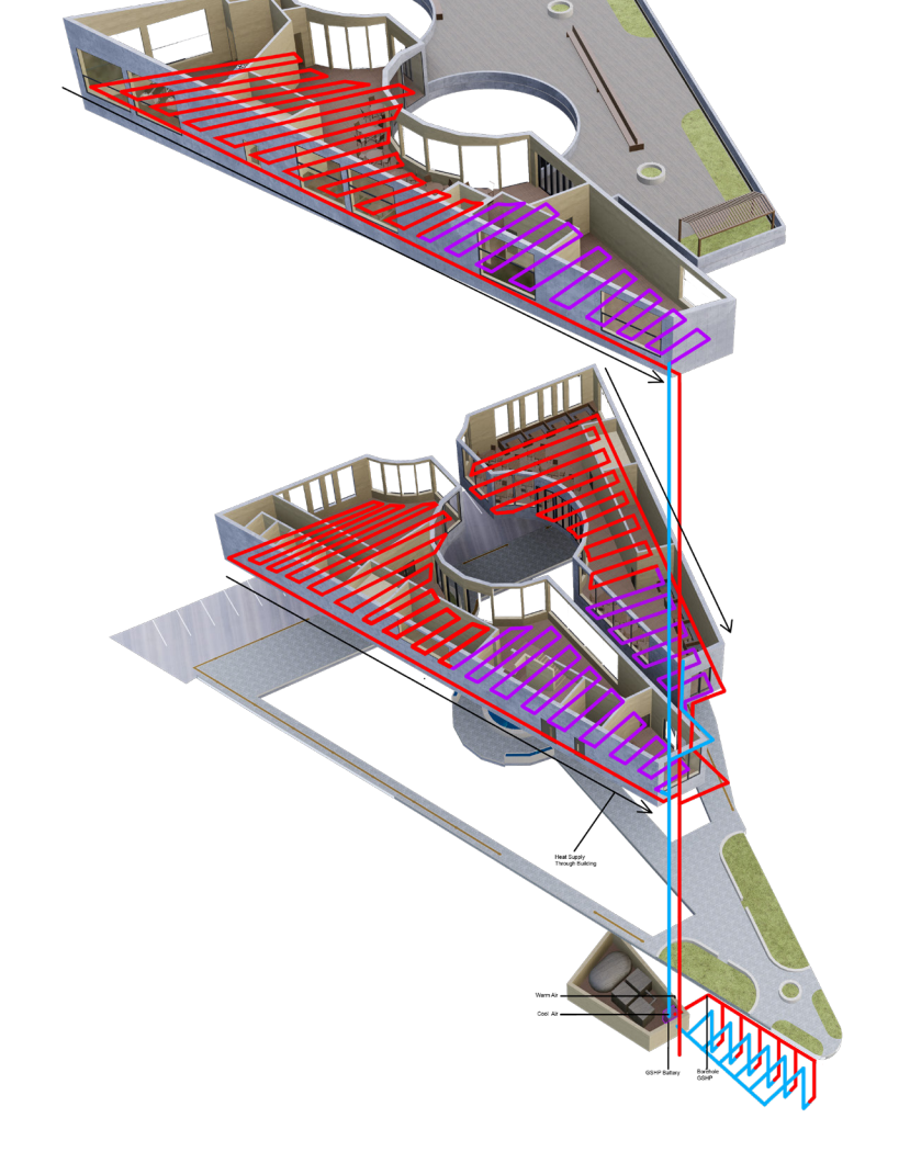
9. Ground Source Heat Pump
