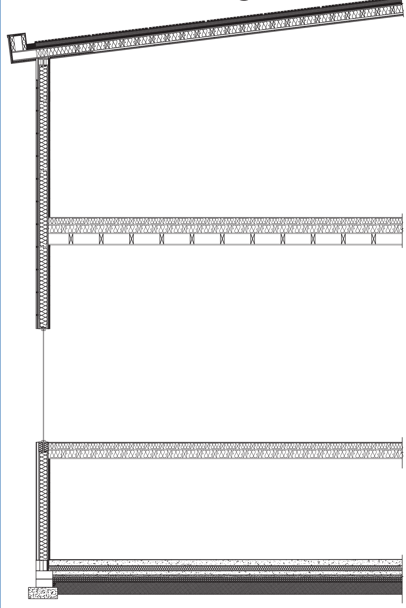
Community Centre Building Detail 1:50 @ A2
