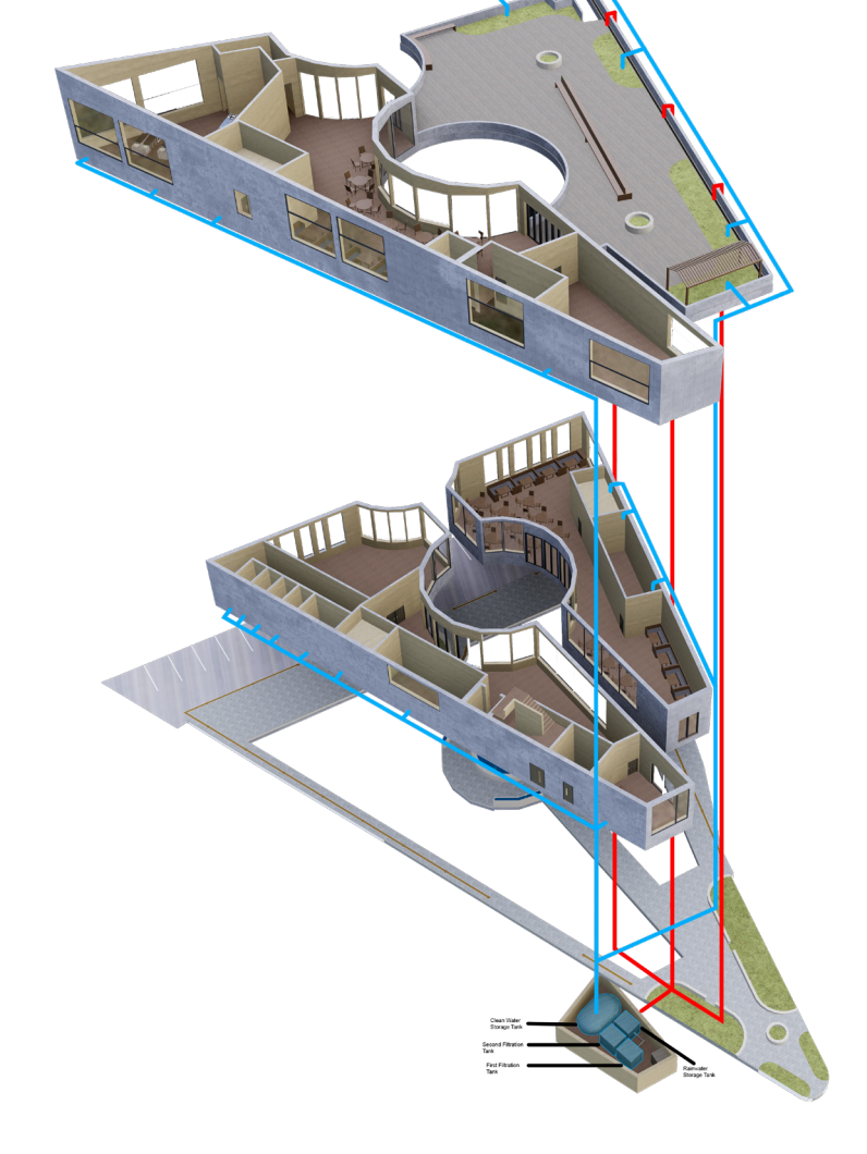
8. Rainwater Collection
