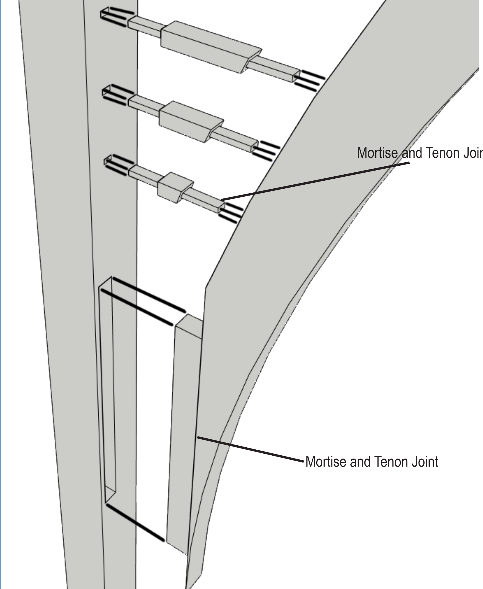
Community Centre Building Detail 1:50 @ A2
